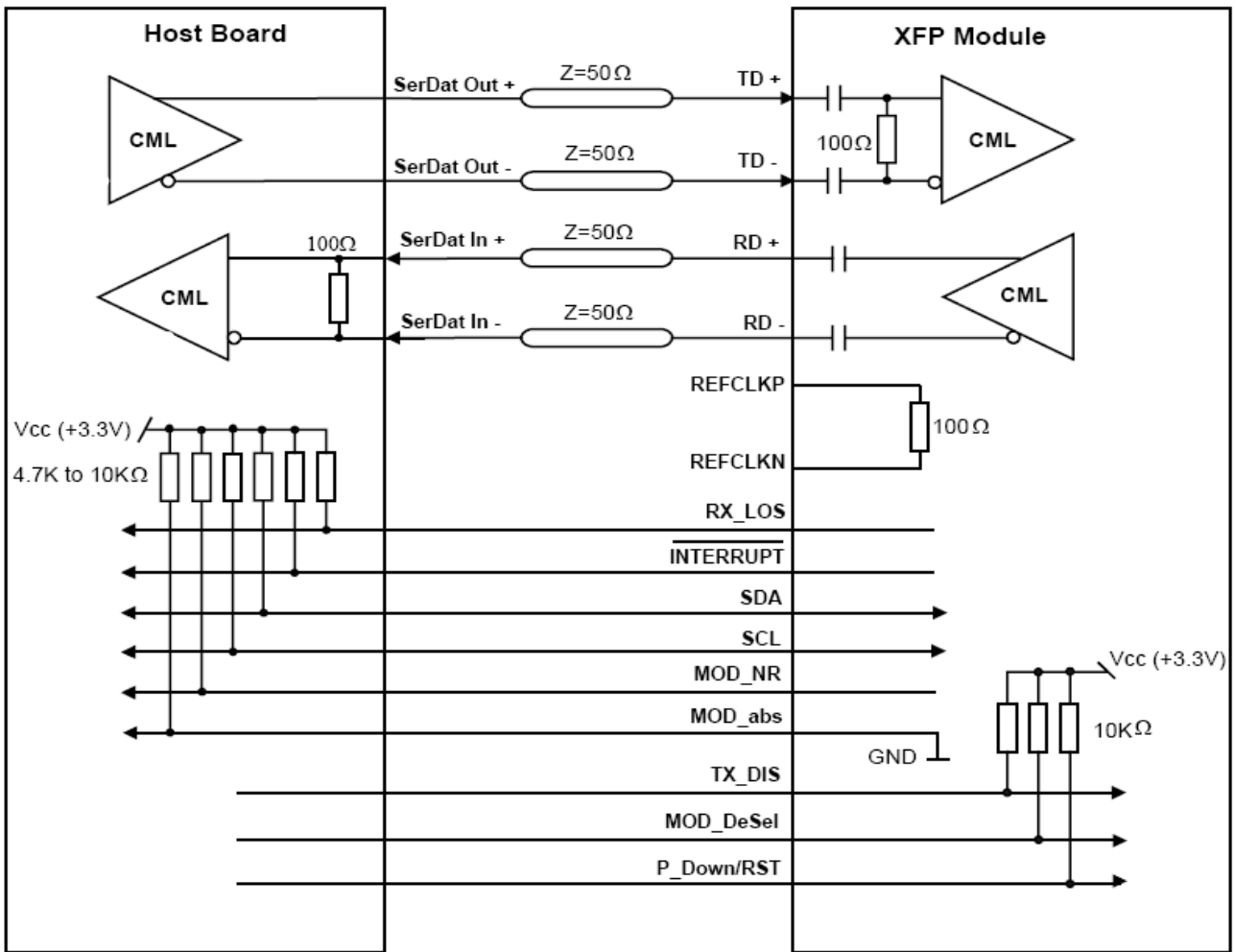
Recommended High-speed Interface Circuit
